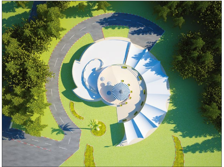
The organic forms of Djanan's architecture are to be created predominantly in earth bag construction. Nylon bags are suspended in a frame at 20 cm intervals, filled with clay from above and then pressed tight. Clay as well as raffia or wire mesh are also used for the upper plaster – all of them inexpensive materials. © all pictures by Kautz-Vella
