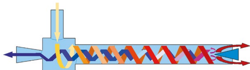
Fig. 9) The Ranque-Hilsch vortex tube is a device without moving parts, with which gas can be divided into a hot and a cold flow. Pressurized gas is injected tangentially into a vortex chamber and is set into a fast rotation (over 1 000 000/min). Due to the high centrifugal forces and other processes that are not yet fully understood, the gas stream is divided into an outer hot and an inner cold stream. The vortex tube was invented in 1933 by the French physicist Georges J. Ranque. The German physicist Rudolf Hilsch improved the design.
