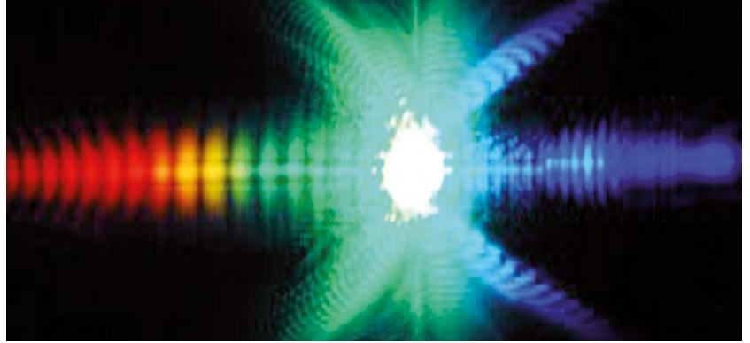
Fig. 5) Image of a "conical wave" from the field of non-linear optics
