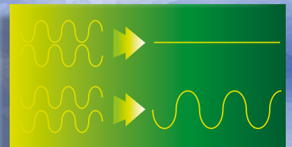
Fig. 3) In-phase waves reinforce each other, opposite-phase waves cancel each other out.
